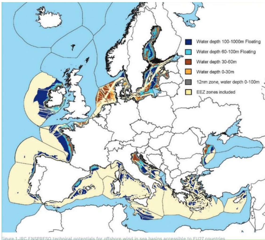
Figure 1. JRC ENSPRESO technical potentials for offshore wind in sea basins accessible to EU27 countries
